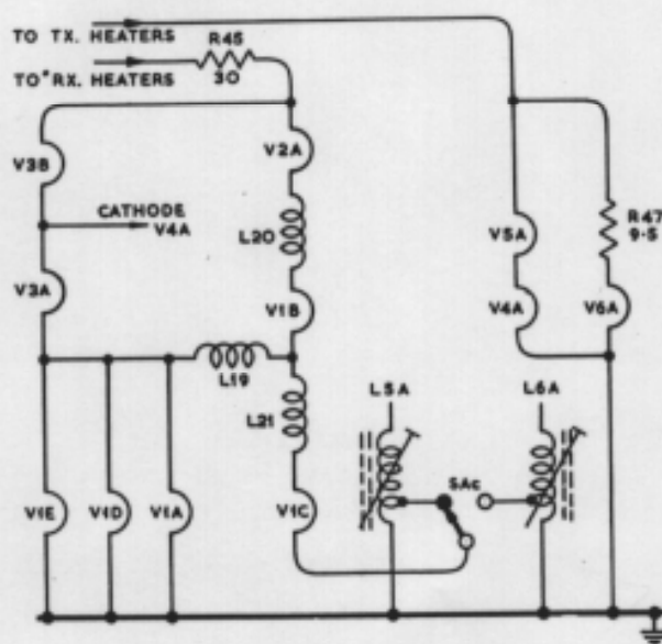
Fig.4 Heater Circuit
