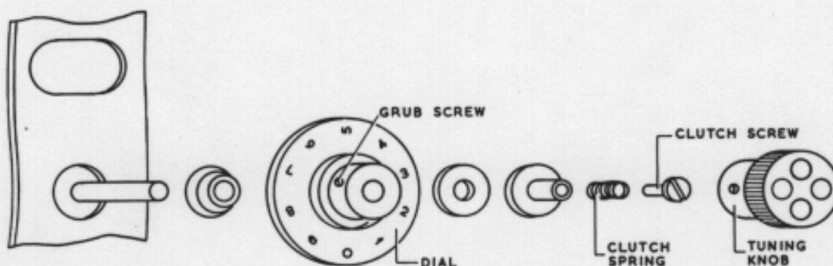
Fig. 12 Dismantling of Aerial Tuning Inductance
