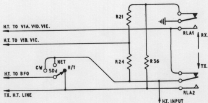
Fig. 5 Transmit/Receive Switching
